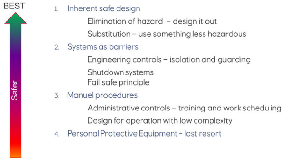
Figure 9 - Safety in design principles
